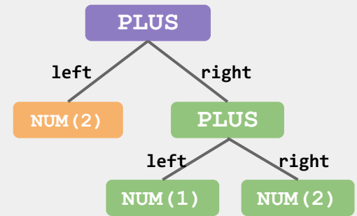
Abstract Syntax Tree
